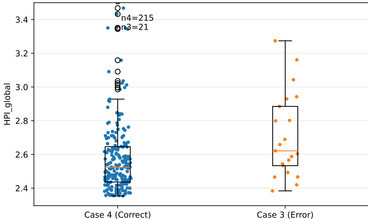
SciBERT: Global HPI distribution (Case 4 vs Case 3)
