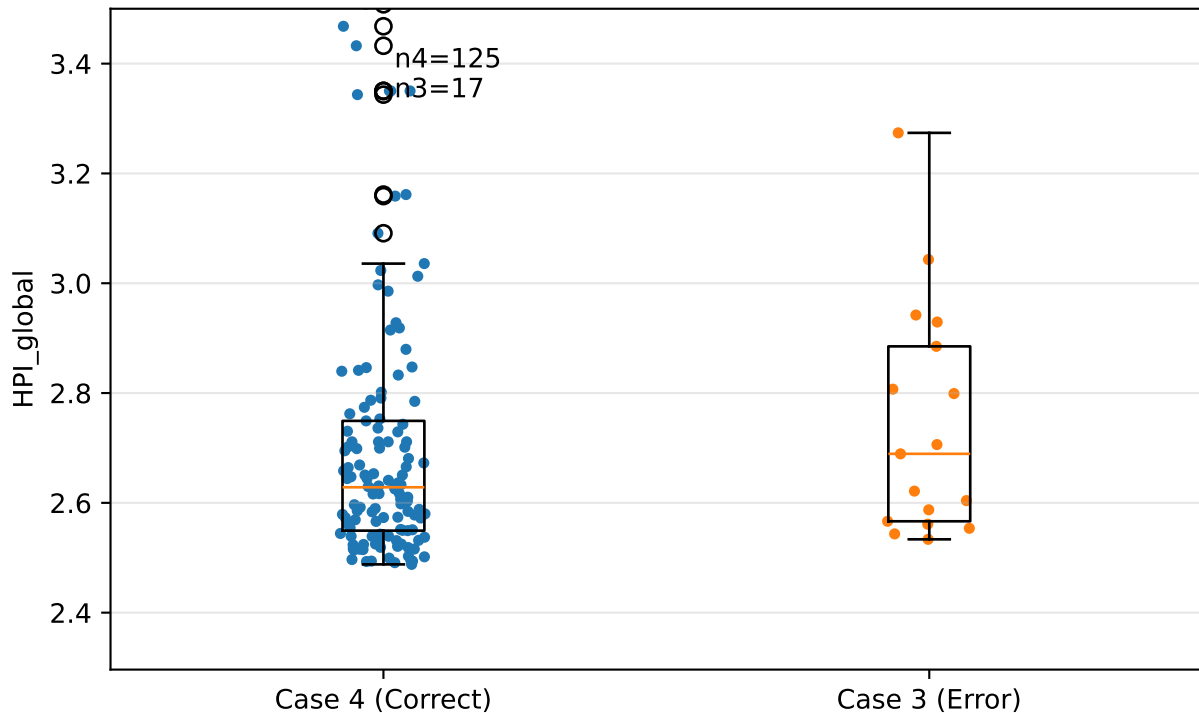
T5: Global HPI distribution (Case 4 vs Case 3)
