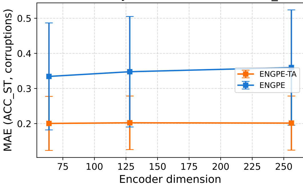
BREEDS entity30 — Ablation: encoder_dim
