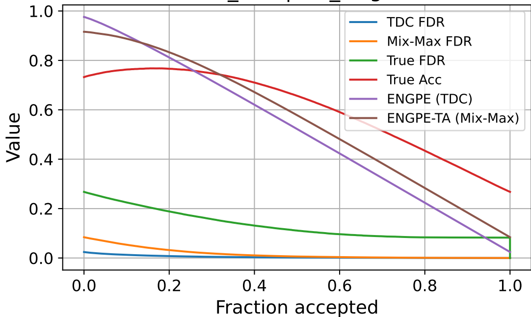
enc_256 | val_target
