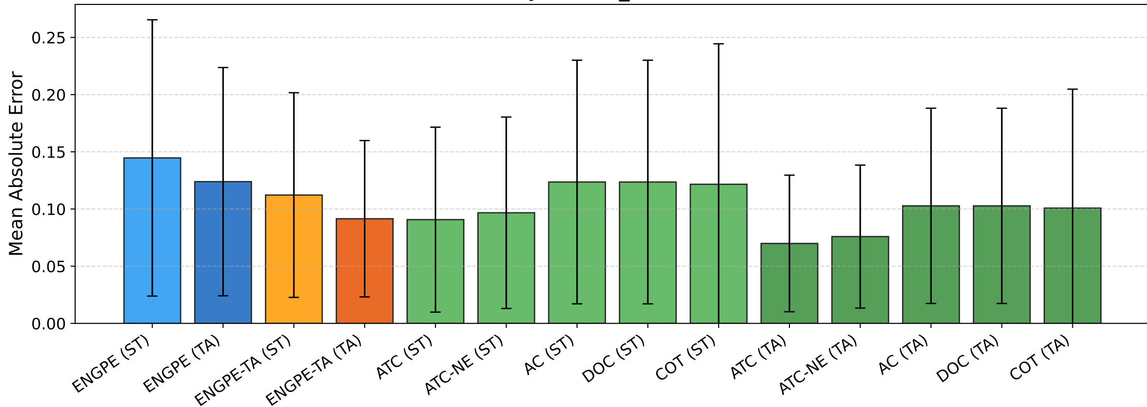
BREEDS entity30 [enc_256] — MAE [clean]
