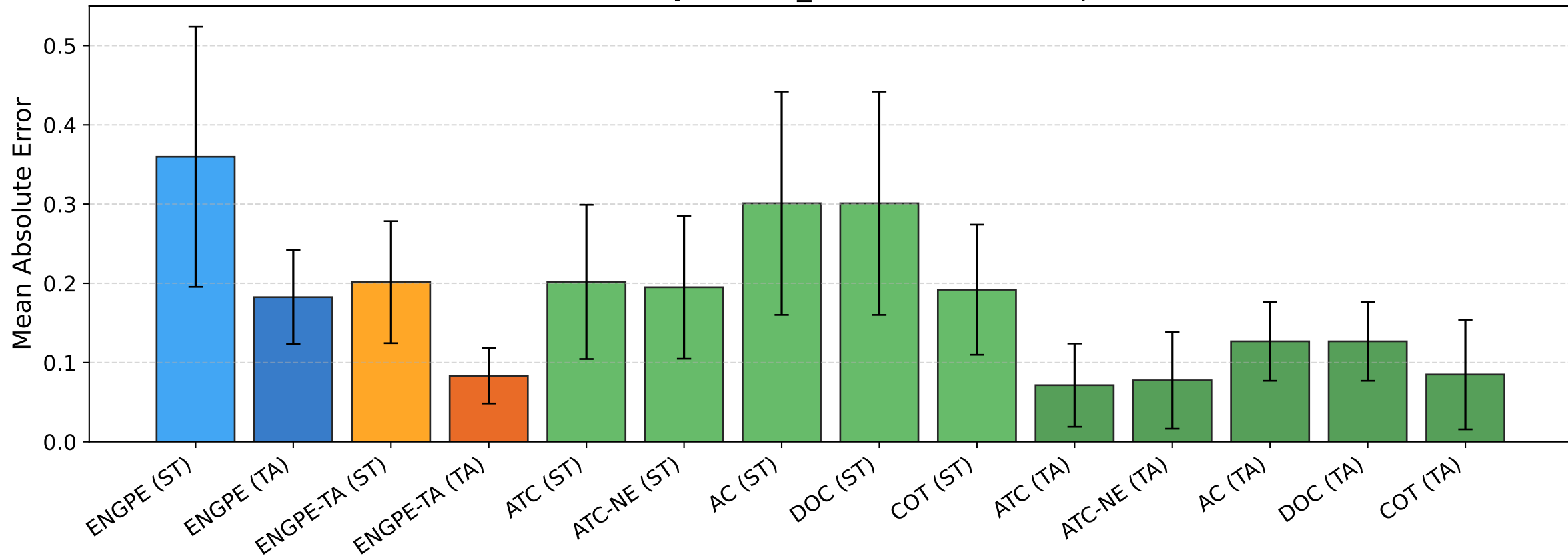
BREEDS entity30 [enc_256] — MAE [corruptions]
