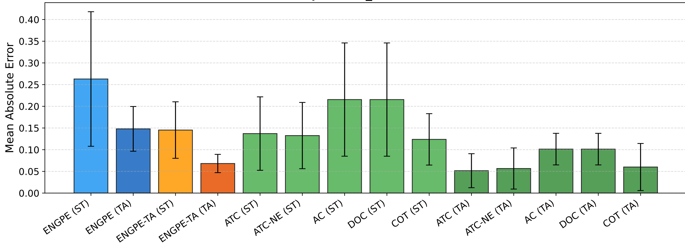
BREEDS entity30 [enc_256] — MAE [source]
