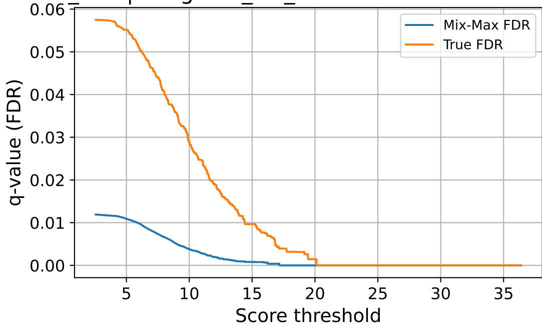
enc_256 | imagenet_val_source — FDR vs Threshold
