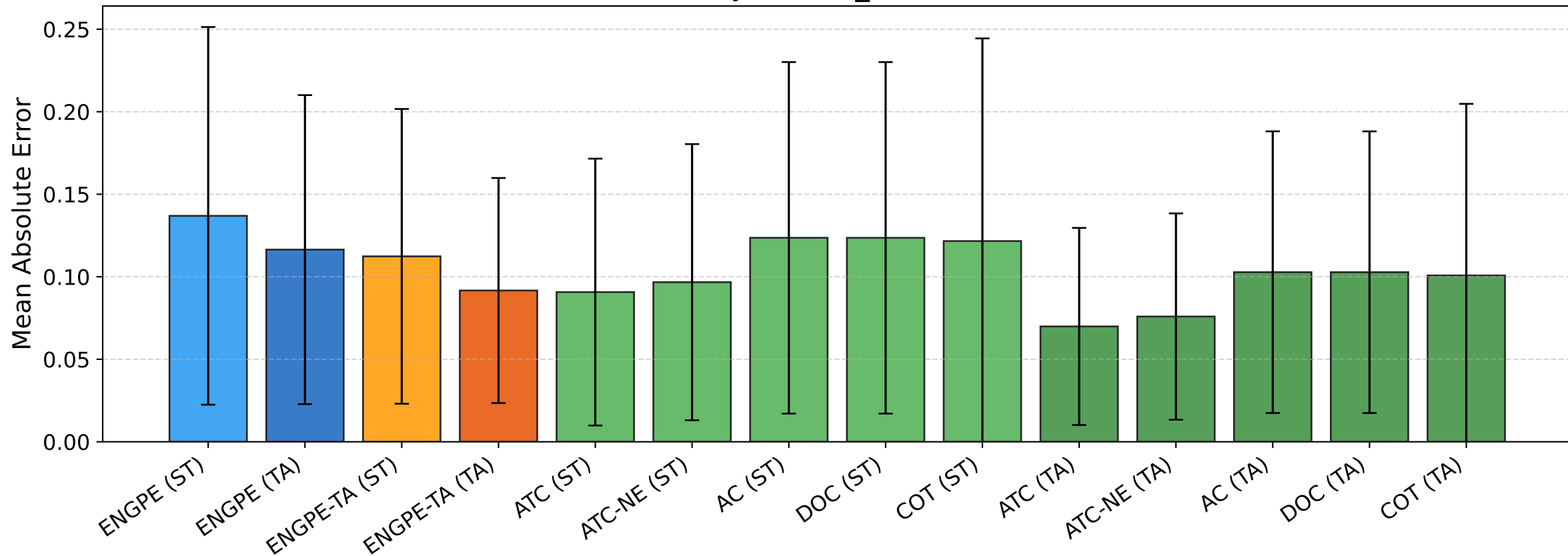
BREEDS entity30 [enc_64] — MAE [clean]
