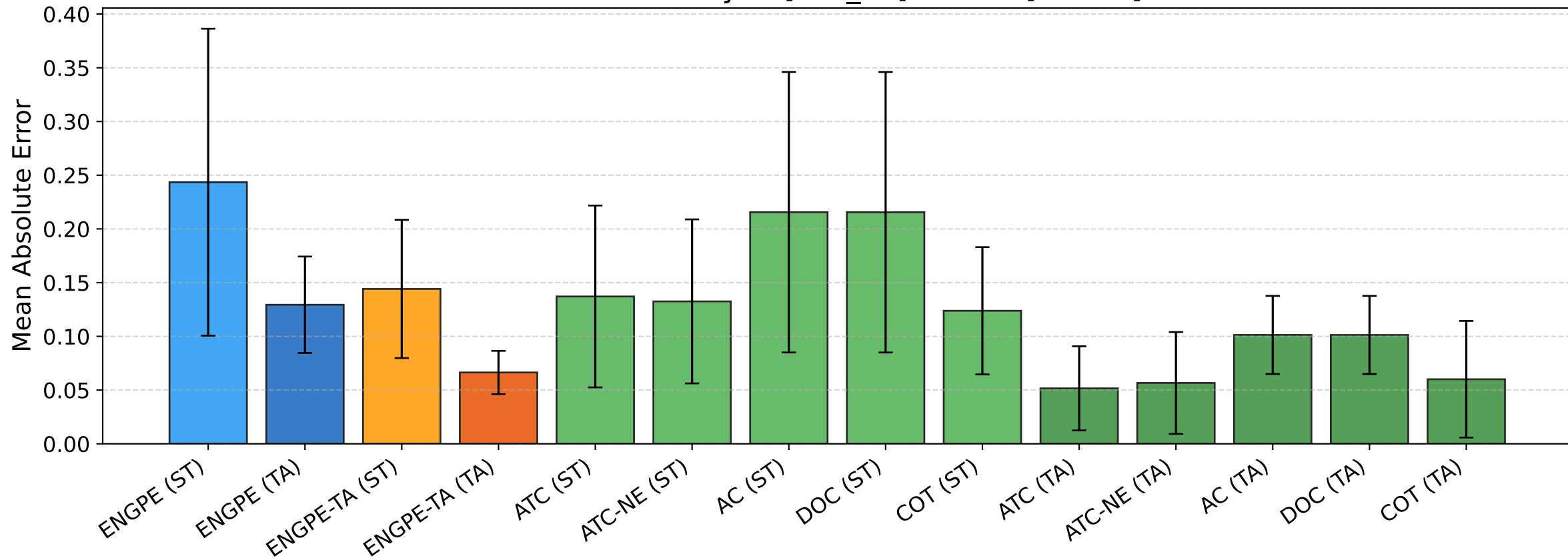
BREEDS entity30 [enc_64] — MAE [source]
