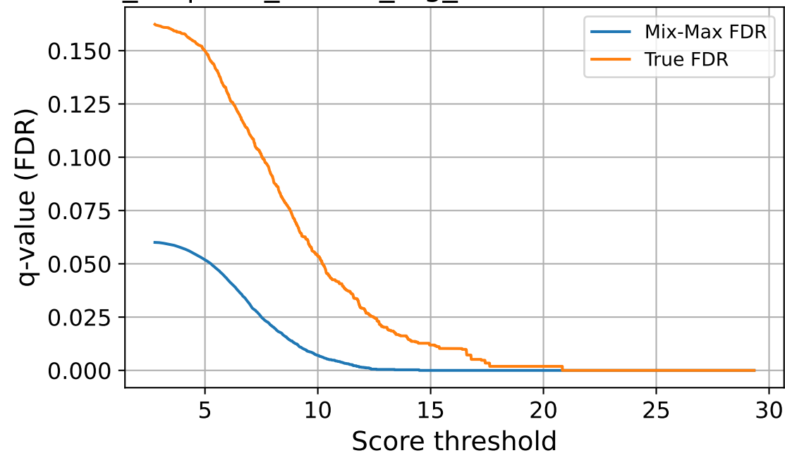
enc_64 | corr_source_fog_sev2 — FDR vs Threshold
