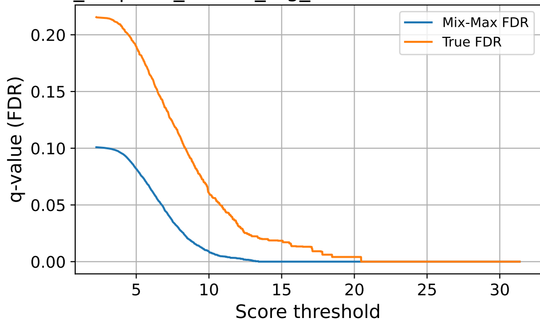
enc_64 | corr_source_fog_sev3 — FDR vs Threshold
