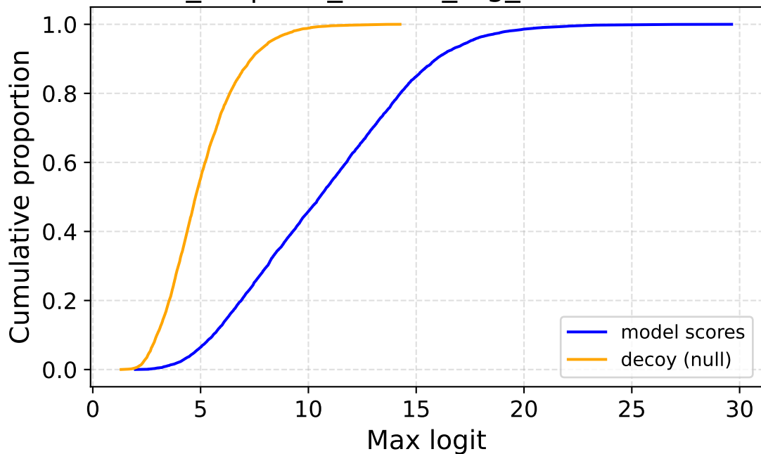
enc_64 | corr_source_fog_sev4 — ECDF
