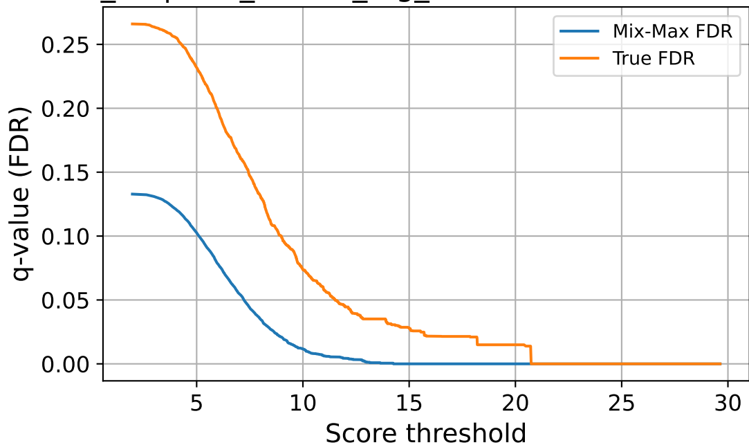
enc_64 | corr_source_fog_sev4 — FDR vs Threshold
