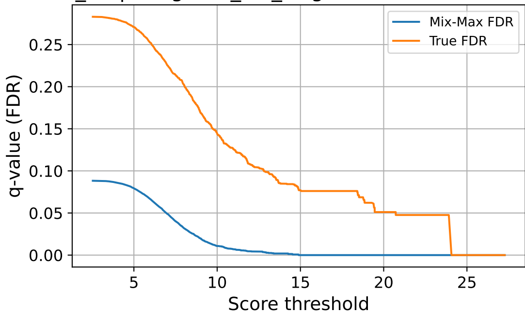
enc_64 | imagenet_val_target — FDR vs Threshold
