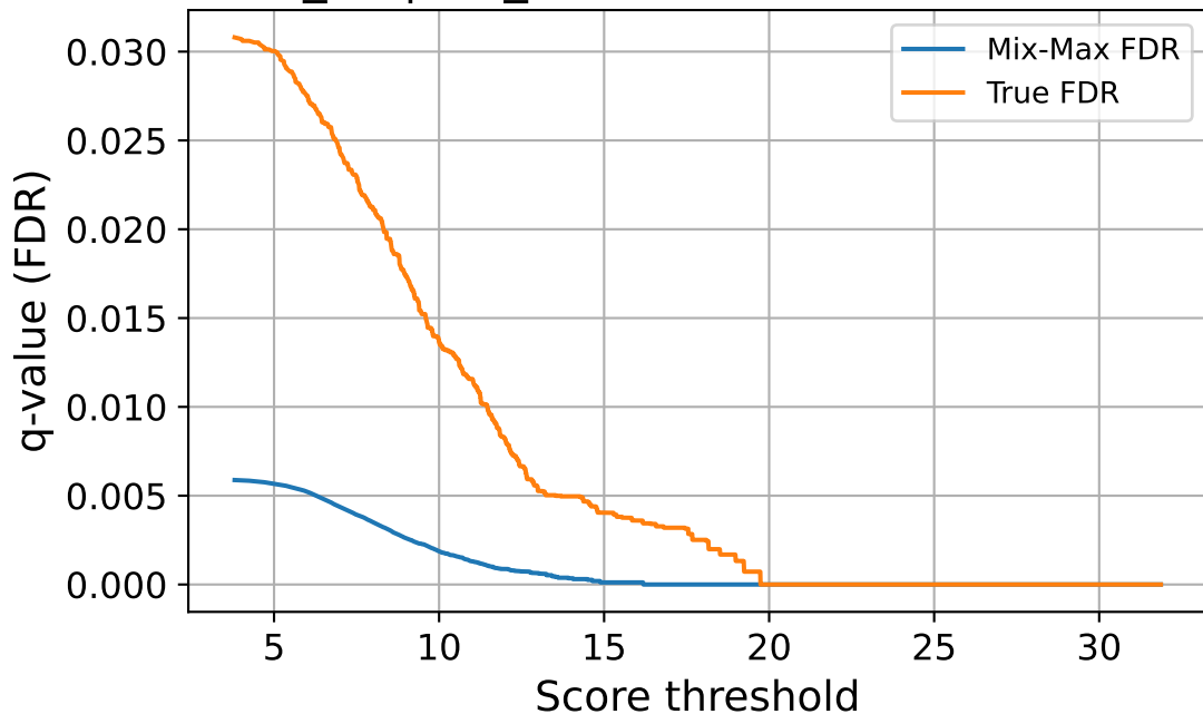
enc_64 | val_source — FDR vs Threshold
