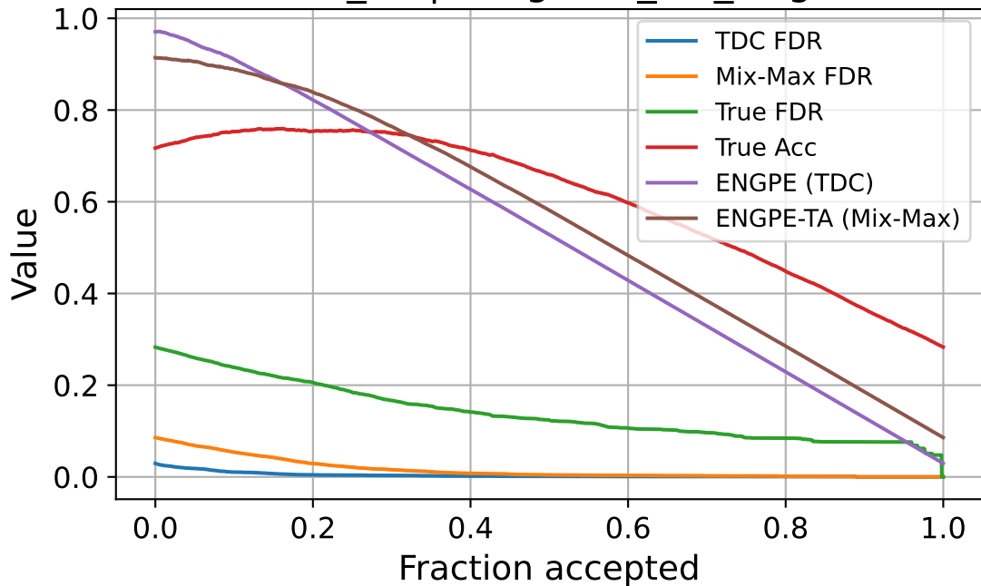
flows_24 | imagenet_val_target
