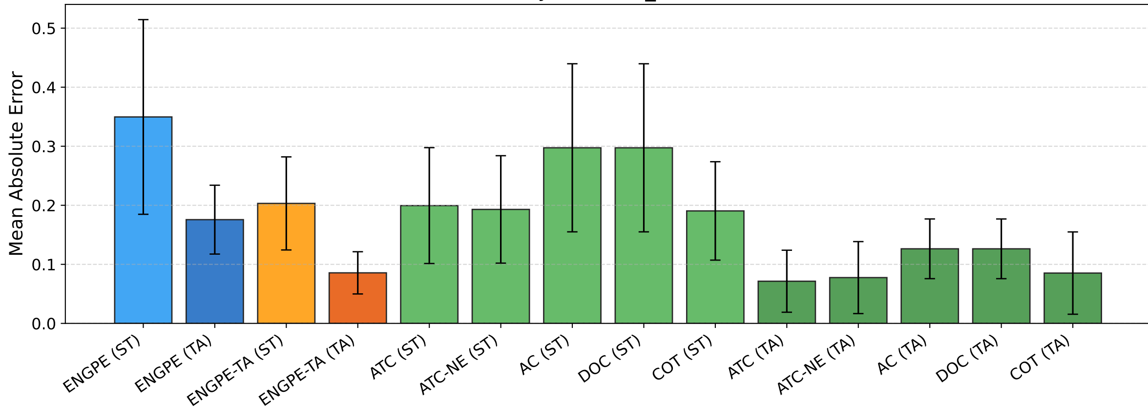
BREEDS entity30 [flows_24] — MAE [all]
