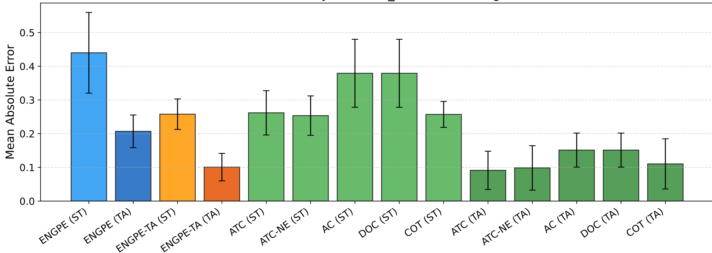
BREEDS entity30 [flows_24] — MAE [target]
