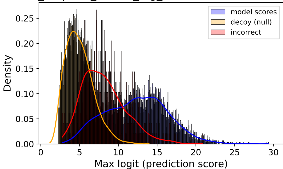
flows_24 | corr_source_fog_sev2 — Score Distribution
