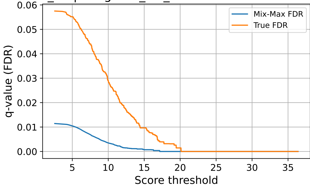
flows_24 | imagenet_val_source — FDR vs Threshold
