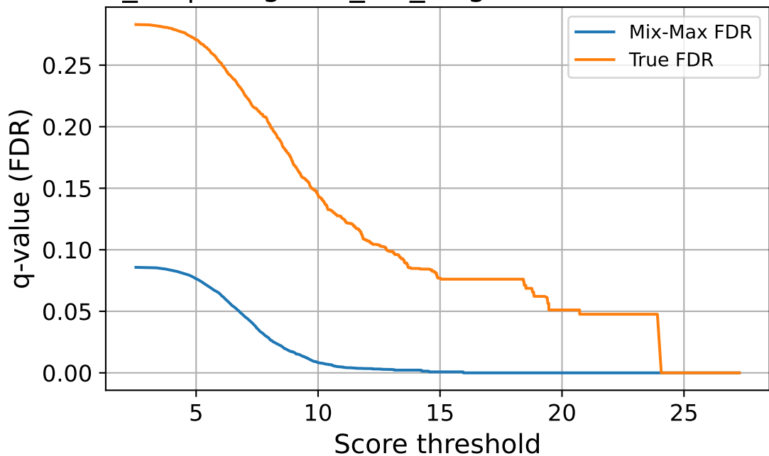
flows_24 | imagenet_val_target — FDR vs Threshold
