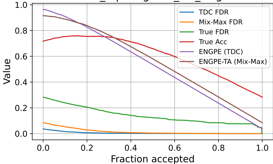
flows_6 | imagenet_val_target
