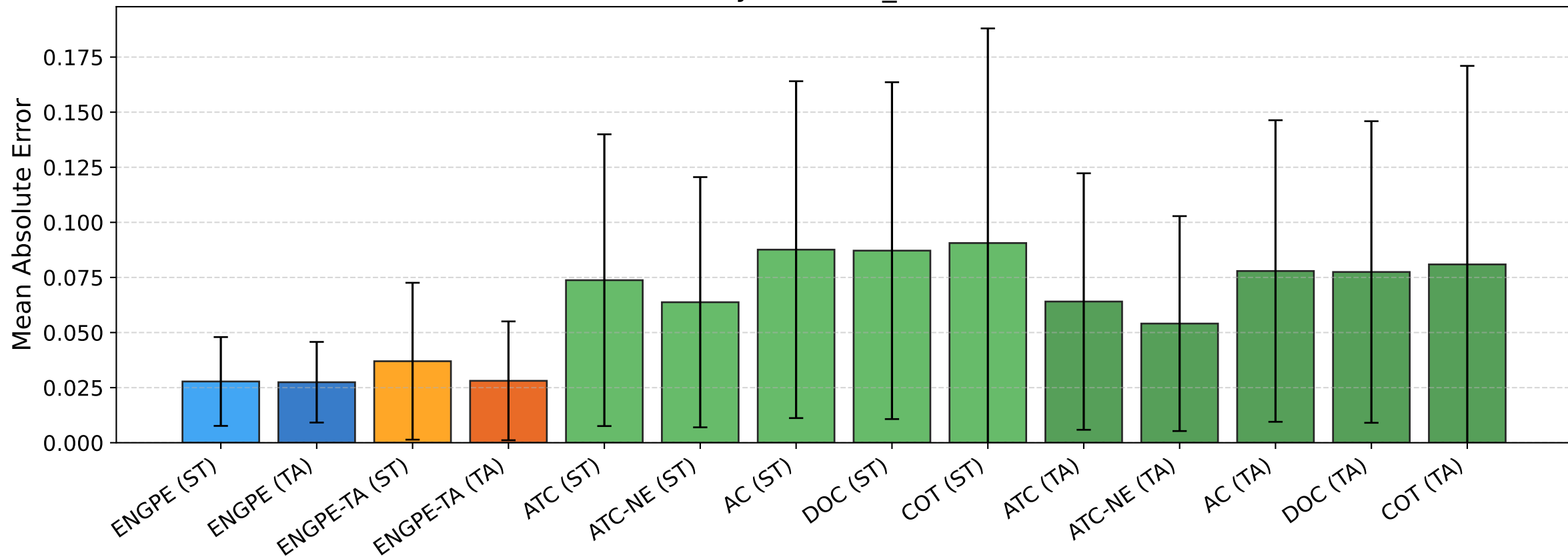
BREEDS entity13 [flows_6] — MAE [clean]
