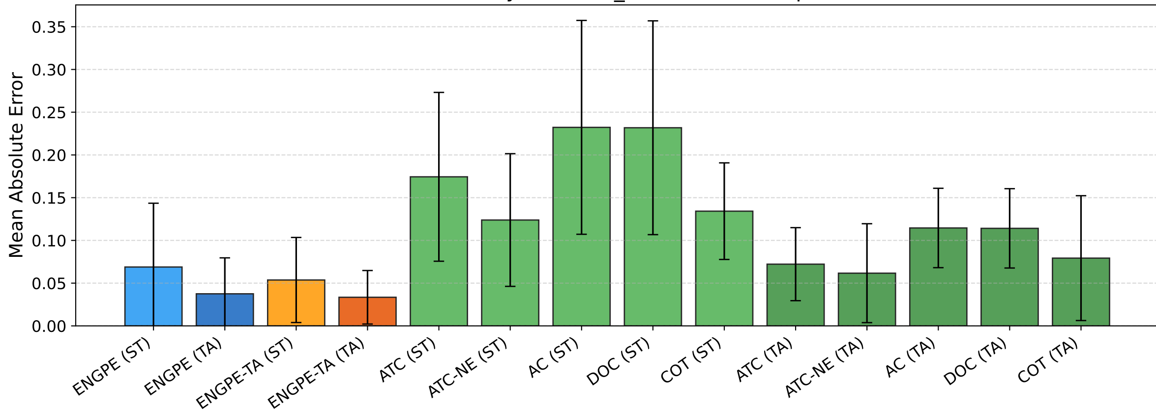
BREEDS entity13 [flows_6] — MAE [corruptions]
