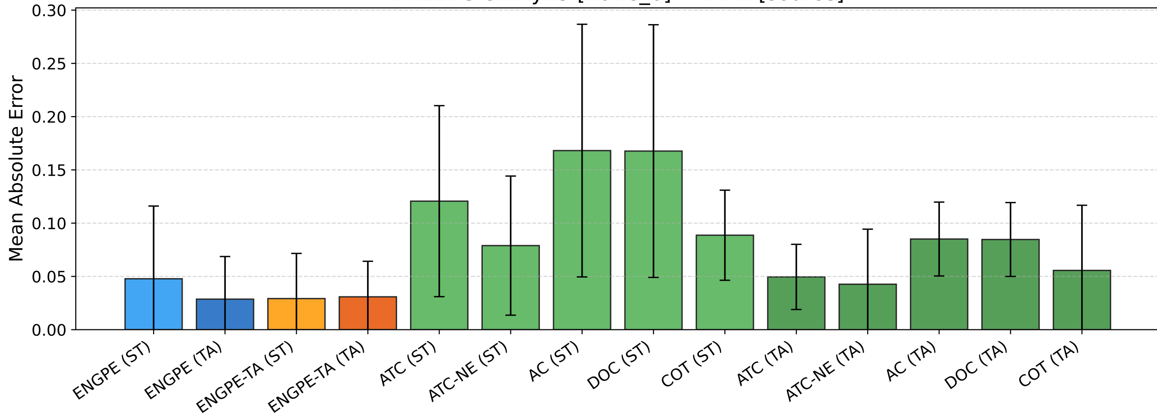
BREEDS entity13 [flows_6] — MAE [source]
