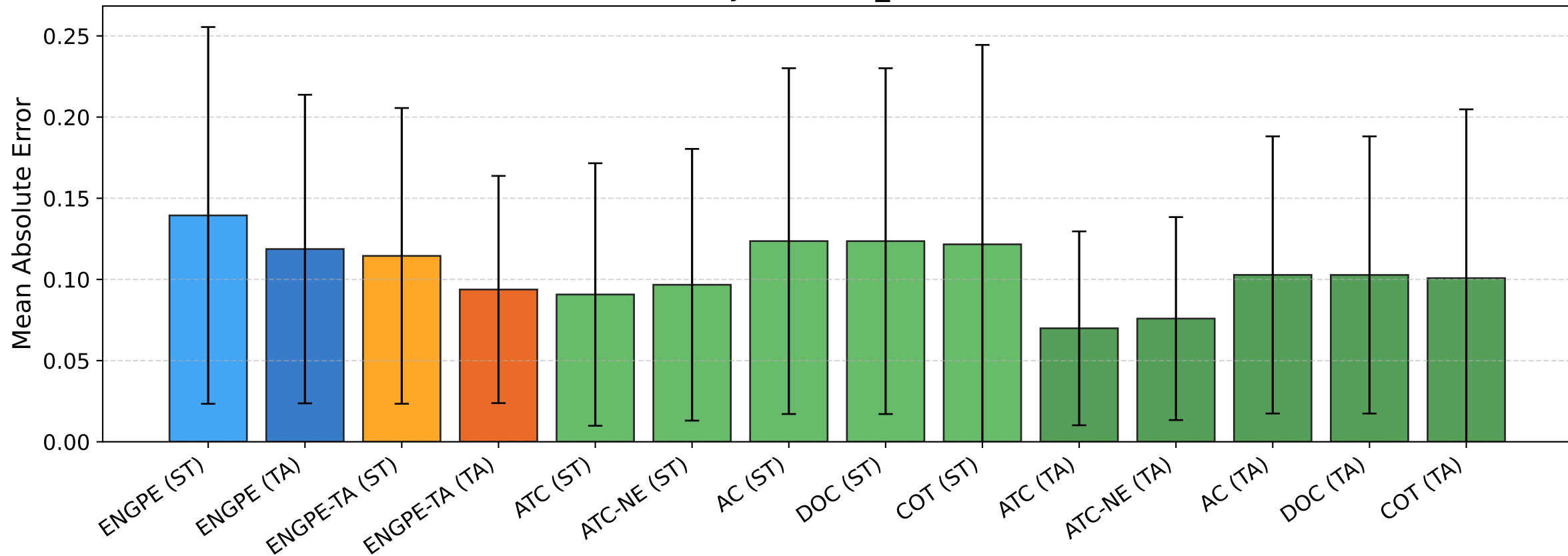
BREEDS entity30 [flows_6] — MAE [clean]
