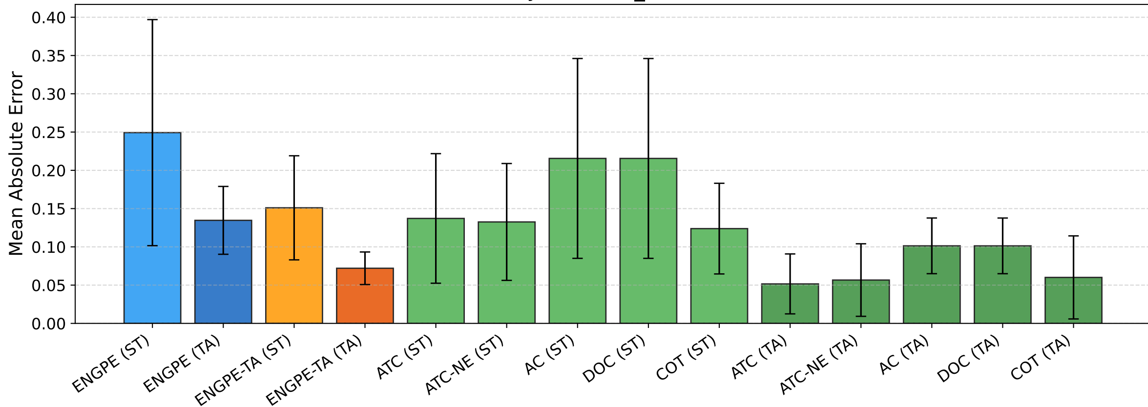
BREEDS entity30 [flows_6] — MAE [source]
