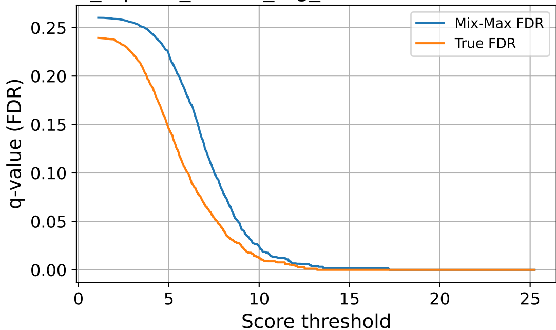
flows_6 | corr_source_fog_sev4 — FDR vs Threshold
