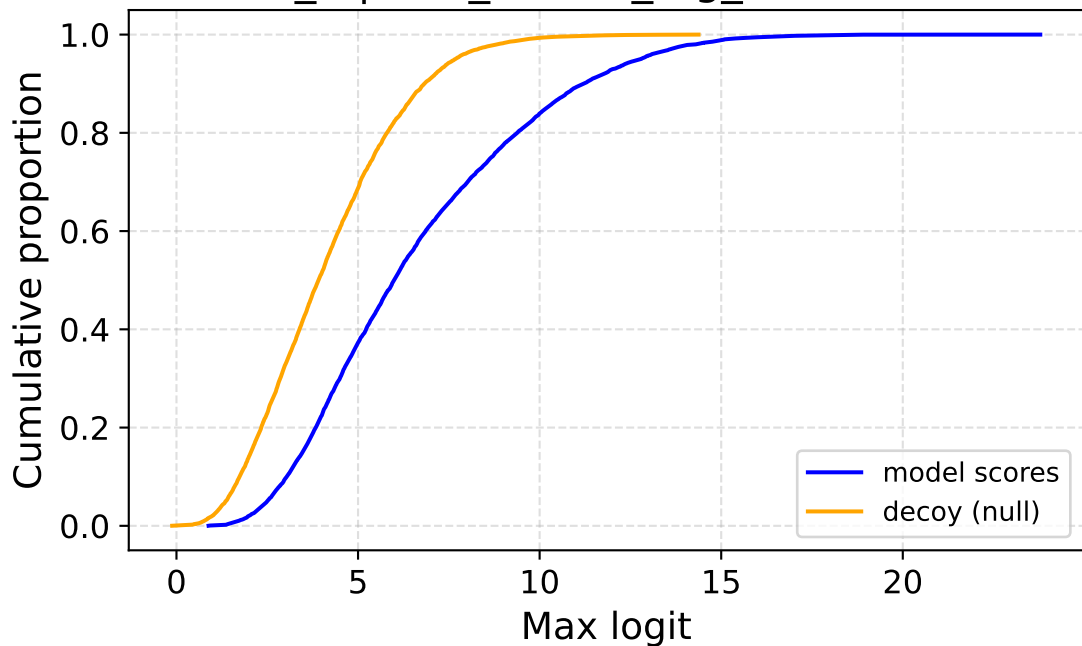
flows_6 | corr_source_fog_sev5 — ECDF
