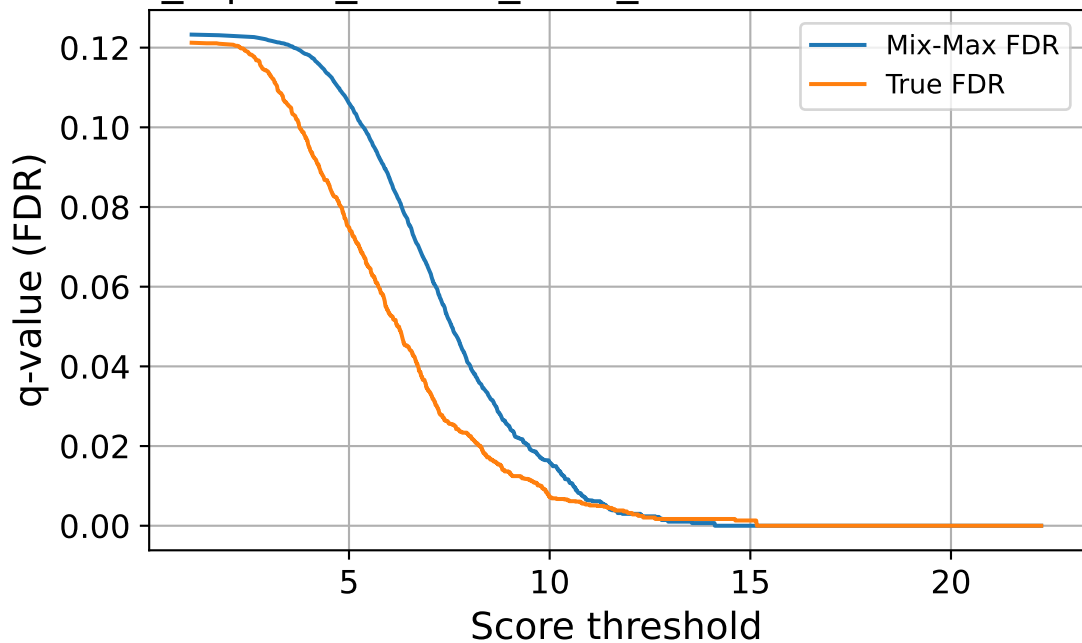
flows_6 | corr_source_frost_sev1 — FDR vs Threshold
