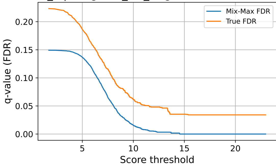
flows_6 | imagenet_val_target — FDR vs Threshold
