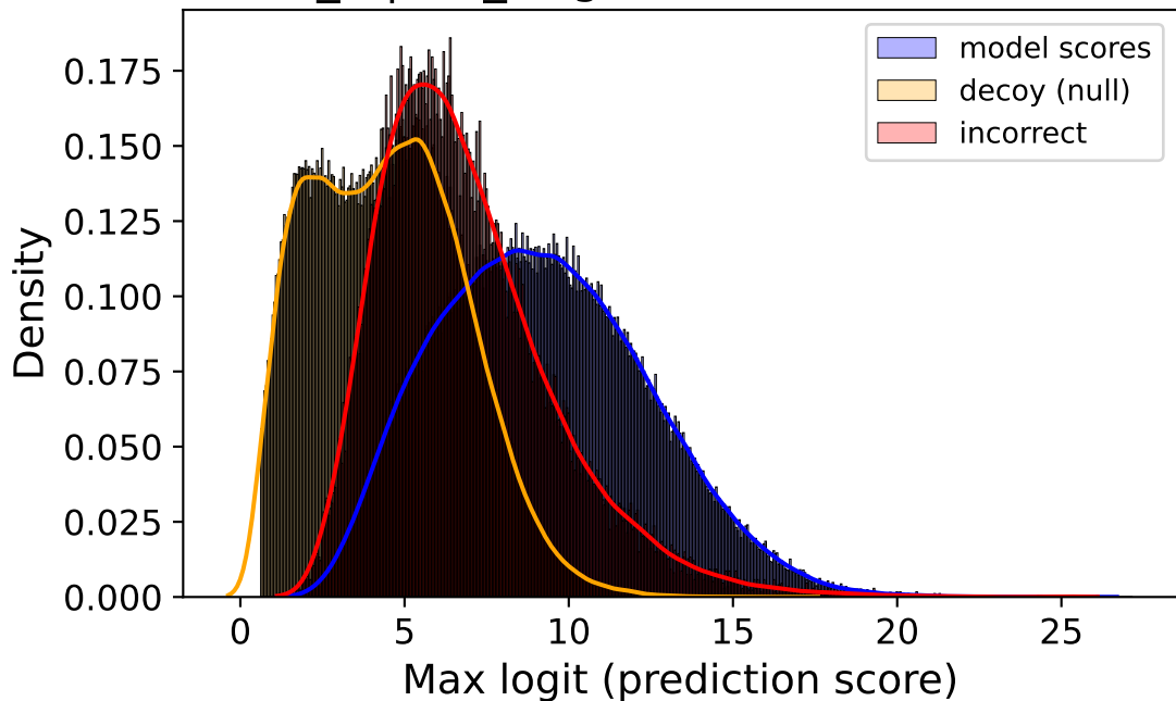
flows_6 | val_target — Score Distributions
