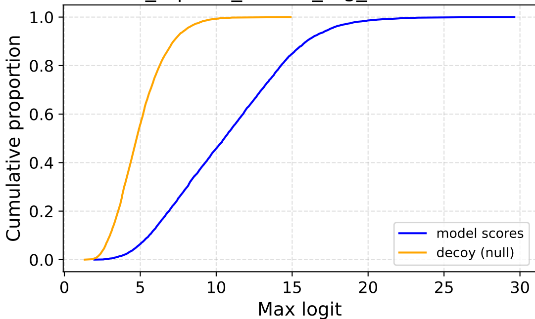
flows_6 | corr_source_fog_sev4 — ECDF
