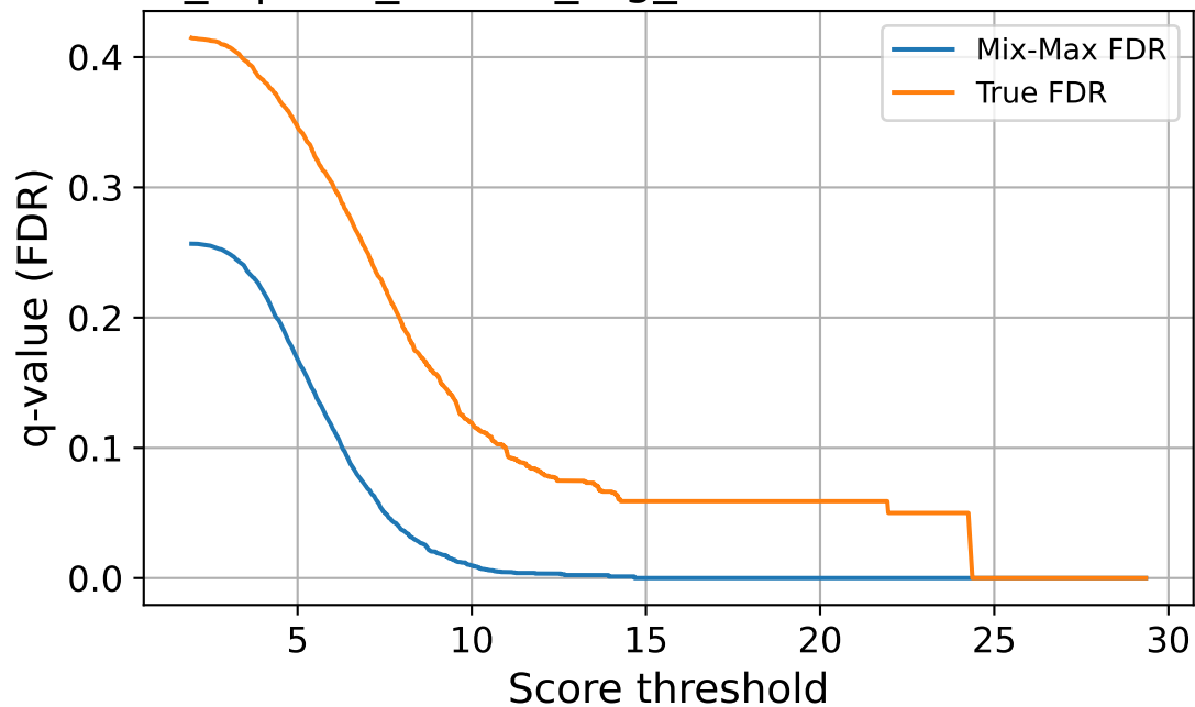
flows_6 | corr_source_fog_sev5 — FDR vs Threshold
