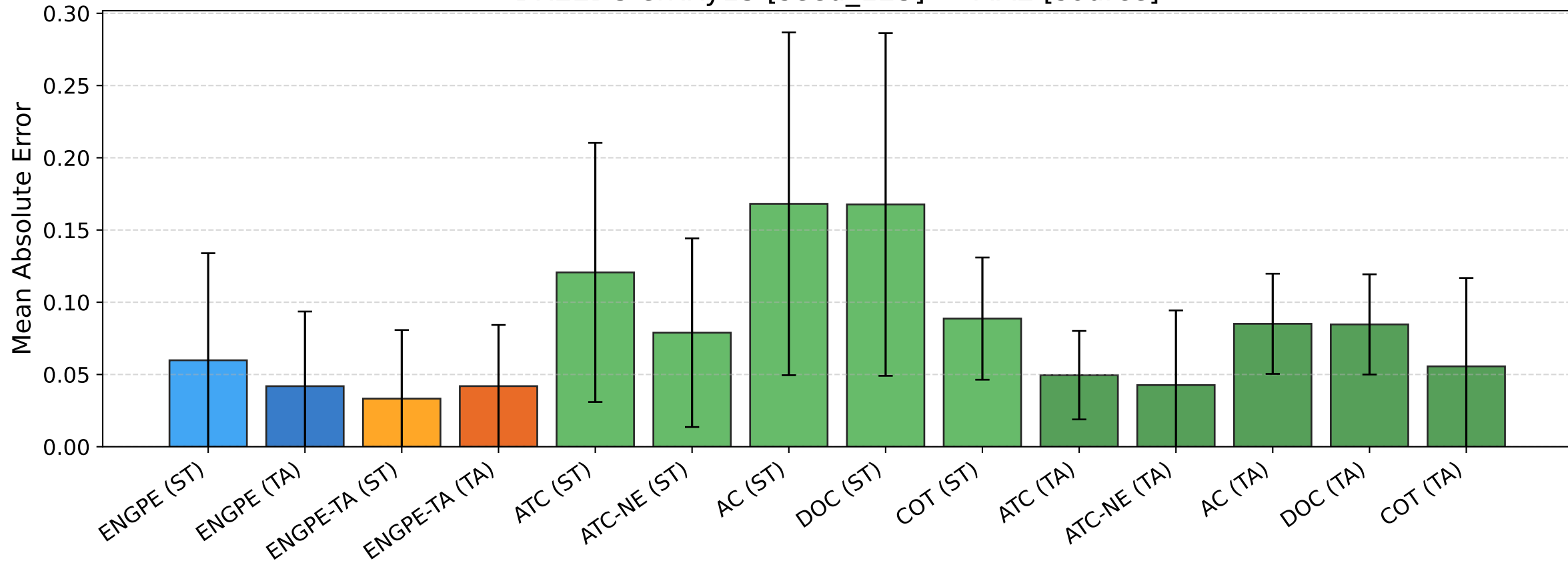
BREEDS entity13 [seed_123] — MAE [source]
