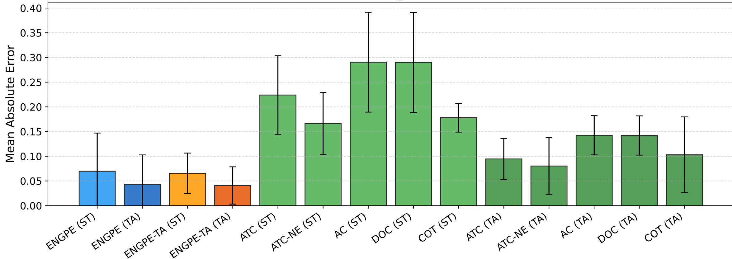
BREEDS entity13 [seed_123] — MAE [target]
