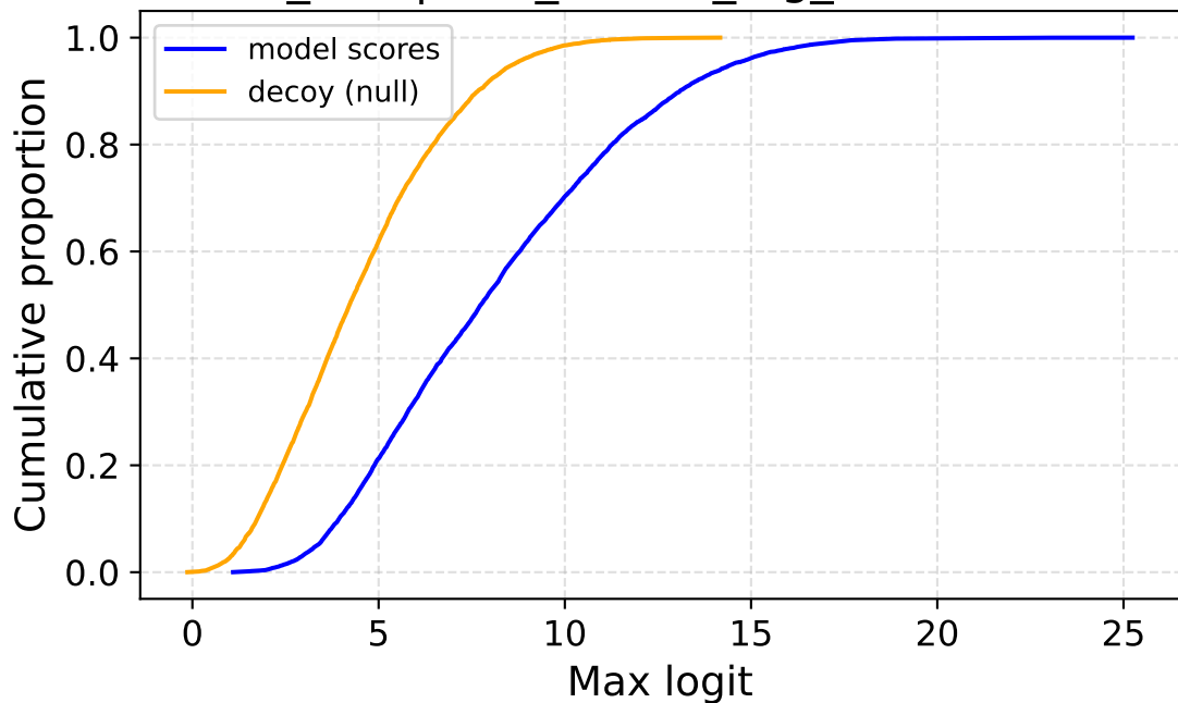
seed_123 | corr_source_fog_sev4 — ECDF
