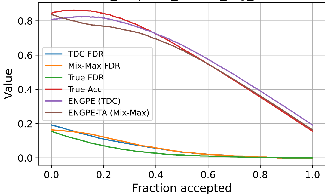
seed_42 | corr_source_fog_sev2
