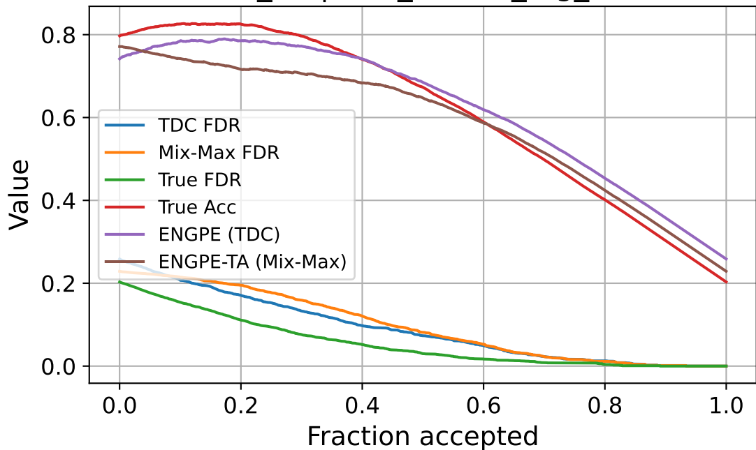
seed_42 | corr_source_fog_sev3
