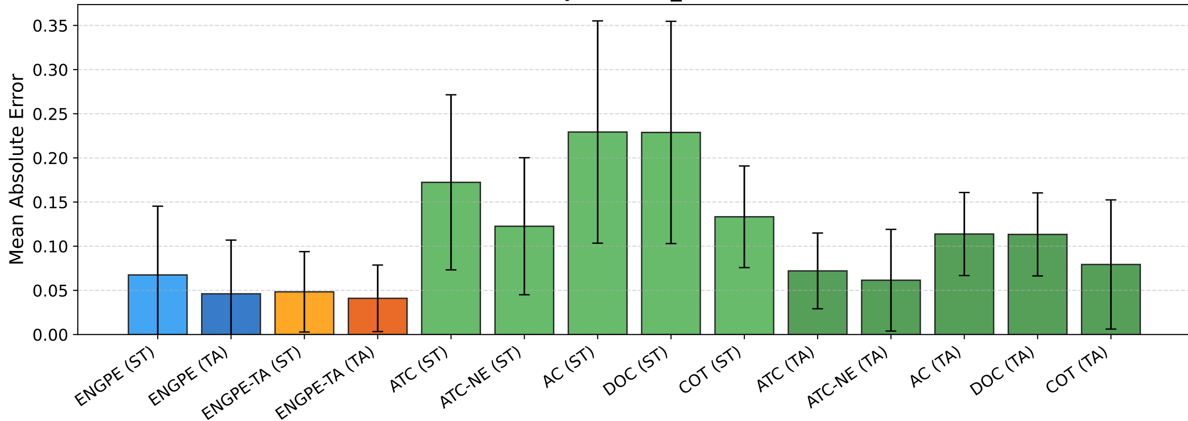
BREEDS entity13 [seed_42] — MAE [all]
