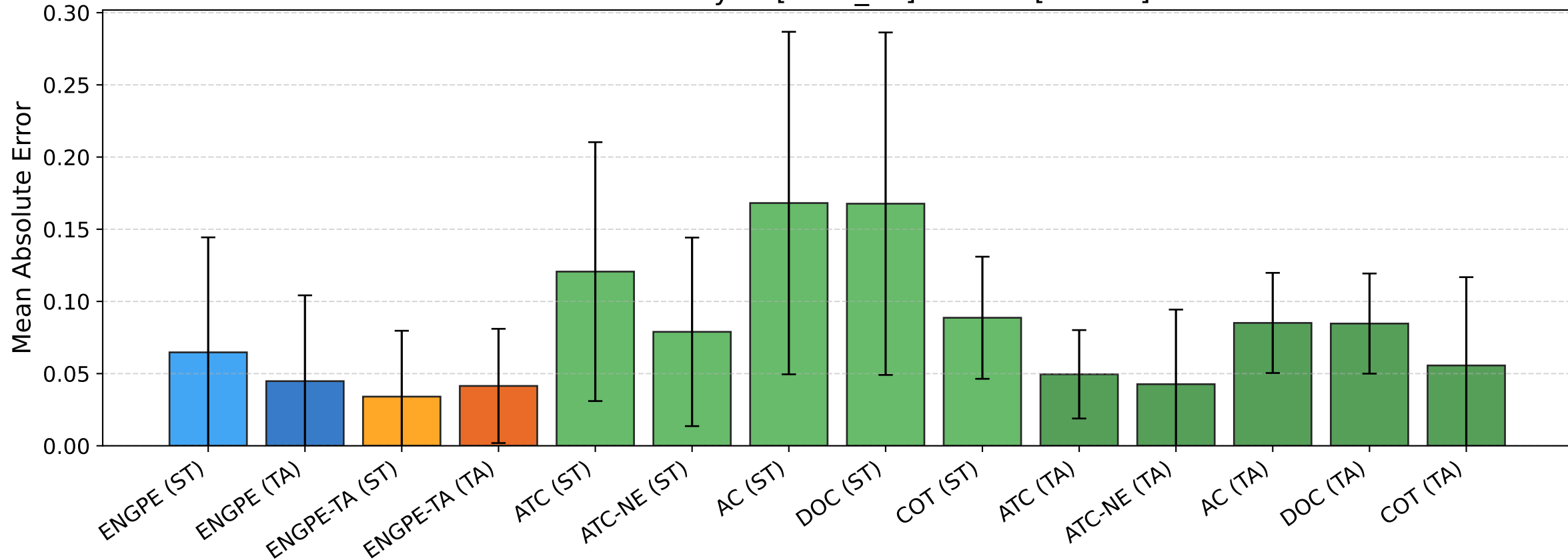
BREEDS entity13 [seed_42] — MAE [source]
