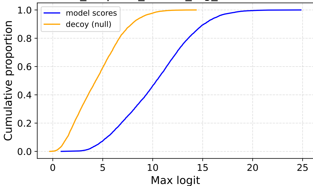
seed_42 | corr_source_fog_sev1 — ECDF
