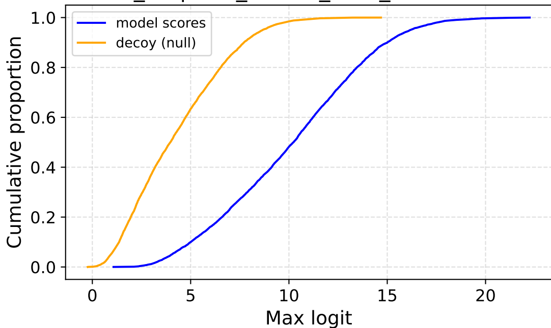
seed_42 | corr_source_frost_sev1 — ECDF
