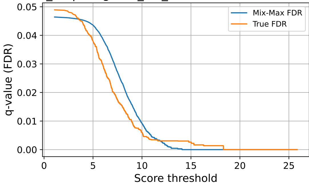
seed_42 | imagenet_val_source — FDR vs Threshold
