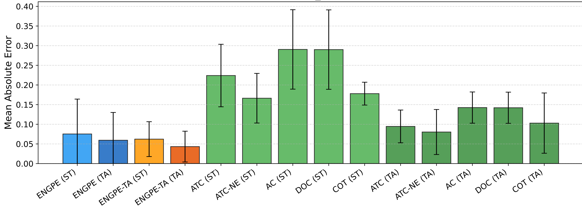
BREEDS entity13 [seed_456] — MAE [target]
