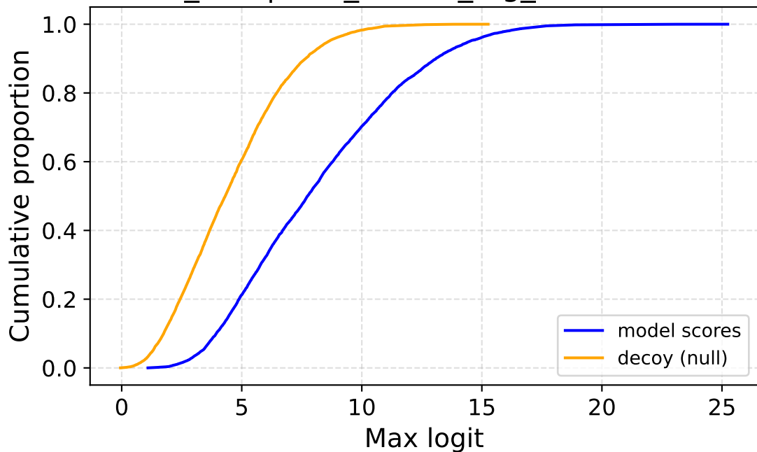
seed_456 | corr_source_fog_sev4 — ECDF
