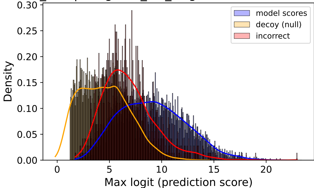
seed_456 | imagenet_val_target — Score Distribution
