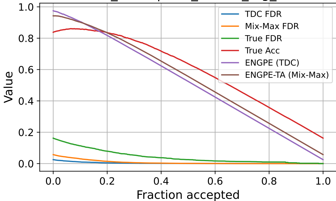
zscore_norm | corr_source_fog_sev2
