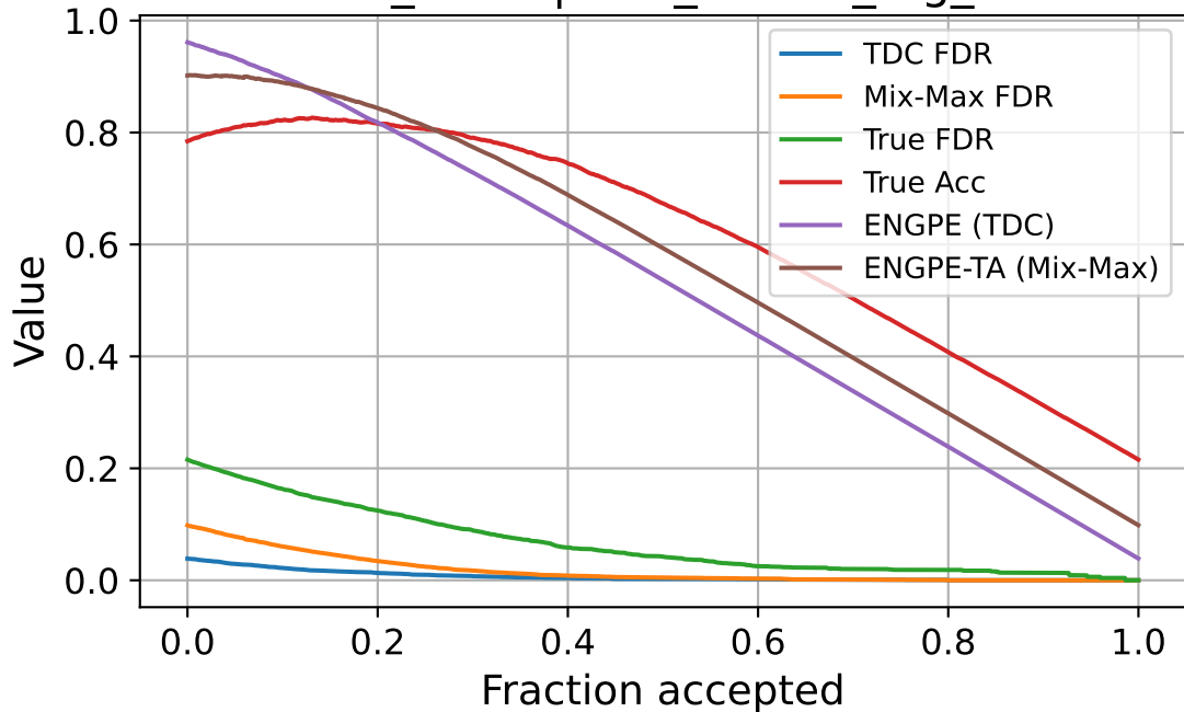
zscore_norm | corr_source_fog_sev3
